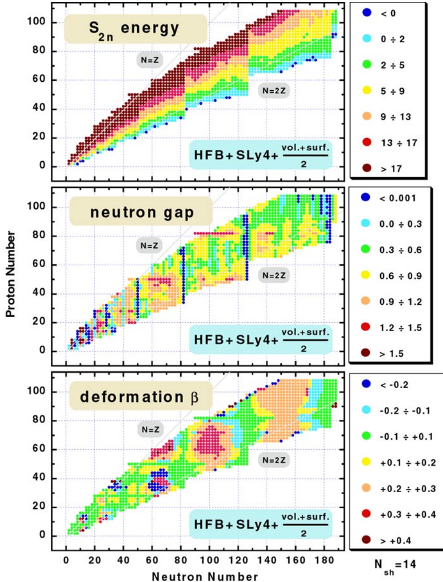
Fig. 5. Results of the HFB + THO + SLy4 deformed calculations for particle-bound even-even nuclei with Z \leq 108 and N \leq 188 .
