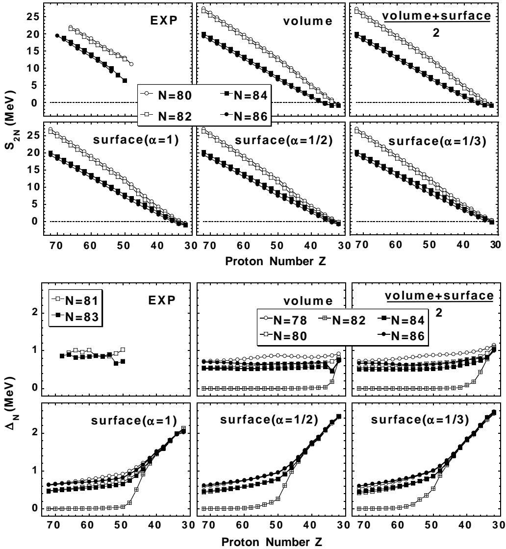
Fig. 4. Comparison between the experimental two-neutron separation energies S_{2N} and neutron pairing gaps \Delta_N (upper left panels, based on masses from ref. [18]), and the corresponding results of the spherical HFB method for the Skyrme SLy4 force [3] and five different versions of the zero-range pairing interaction (see text).
