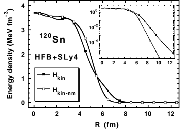
Fig. 2. Microscopic kinetic-energy density \mathcal{H}_{\text{kin}} (full squares) compared to the nuclear-matter (volume) approximation \mathcal{H}_{\text{kin-nm}} (open squares).
