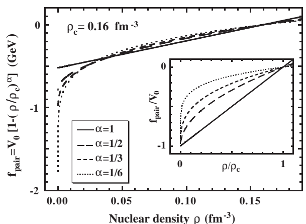
Fig. 3. Radial strength factor f_{\text{pair}} of the density-dependent delta interaction, eq. (14), as a function of \rho = \rho_0 for several values of \alpha . The value of \rho_c was assumed to be 0.16 \text{ fm}^{-3} . At each value of \alpha , the strength V_0 was adjusted to reproduce the neutron pairing gap in ^{120}\text{Sn} . The inset shows f_{\text{pair}}/|V_0| as a function of dimensionless normalized density \rho_0/\rho_c (from ref. [17]).
